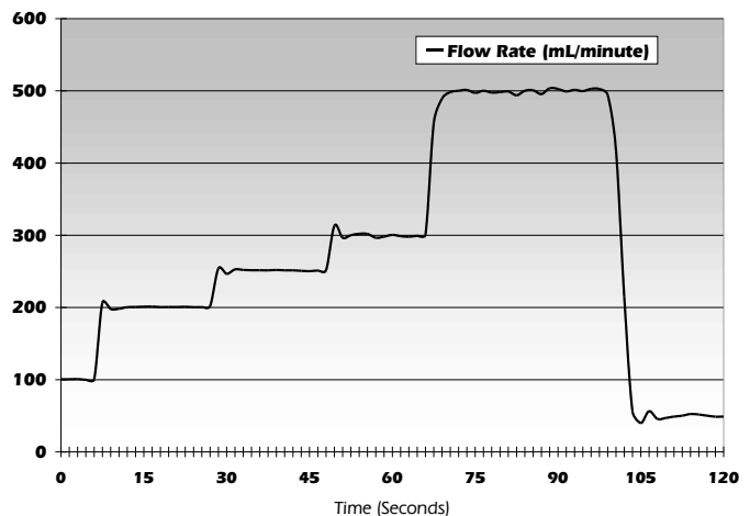
Tests run on a new, randomly chosen McMillan 500 mL/minute (range 5) liquid flow controller on deionized water with 20 psig input pressure.
